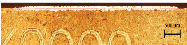
Fig. 3 Image of the flank face of a worn tool ( a_p = 0.05\text{mm} , v_c = 80\text{m/min} )
