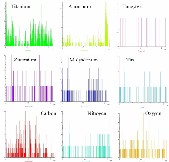
Fig. 8 The EDX line analysis of the worn tool
