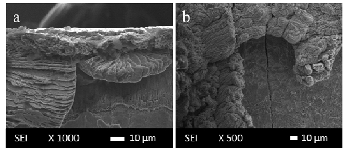
Fig. 4 SEM images of different wear mechanisms. a built-up edge formation, b micro crack formation
