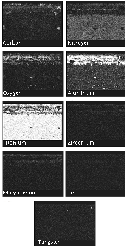
Fig. 10A chemical elements map
