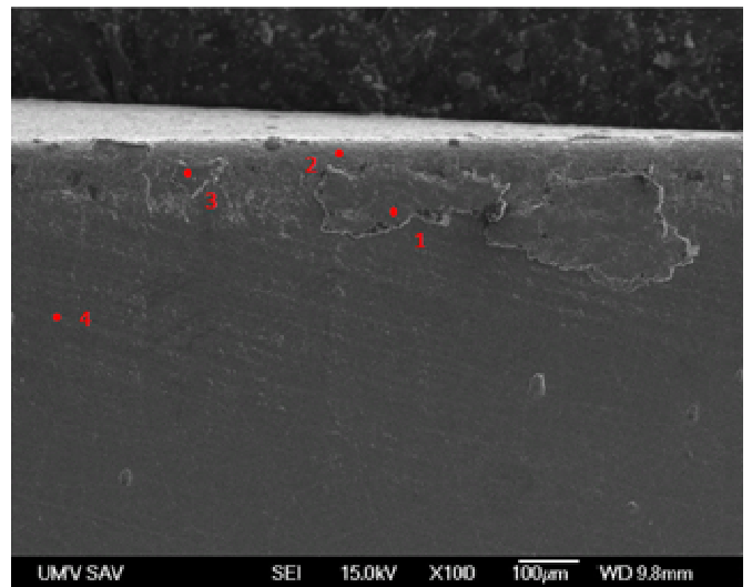
Fig. 5 The EDX point analysis of the worn tool
