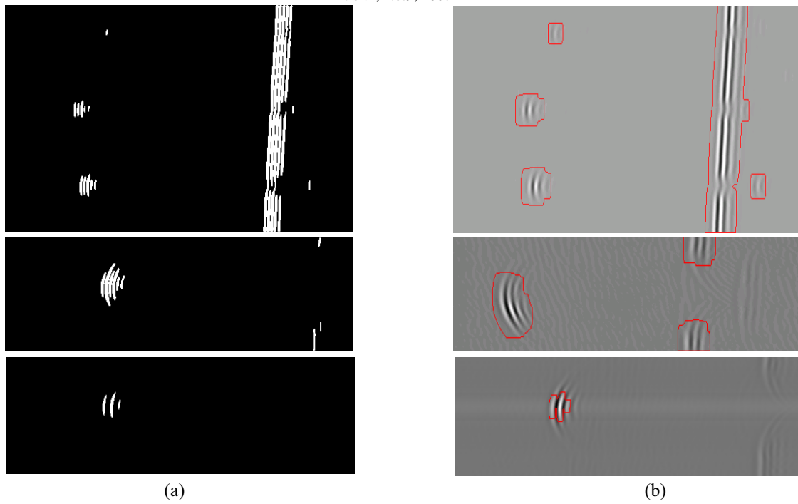
Fig. 5 Segmentation results of laboratory TOFD images
