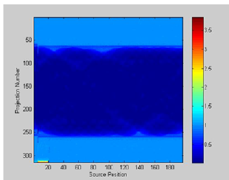
Fig. 4 Image of senogram for pebblebed reactor
