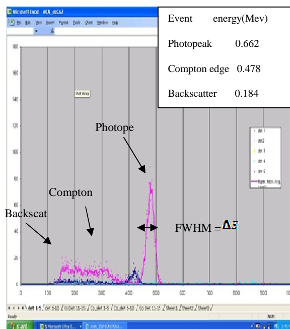
Fig. 2 Spectrum obtaining for isotope Cs-137 from five detectors ,Test No 1
