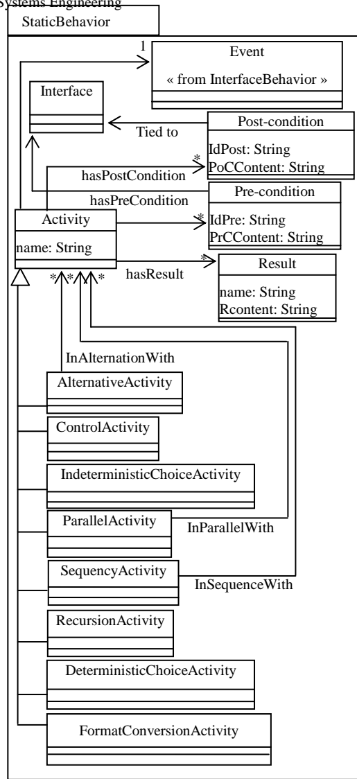
Fig. 2 Package 2: Static behavior meta-model
