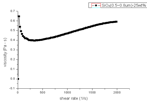
Fig. 2 Viscosity as a function of shear rate for STF1. The shear rate was set from 0/s to 2000/s
