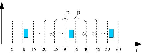
Fig. 2 A case of \langle \overline{p} \rangle \supseteq \binom{1}{p}
