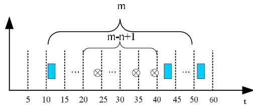
Fig. 1 A case of \langle \overline{m-n+1} \rangle \subseteq \binom{n}{m}
