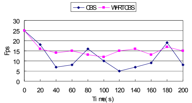
Fig. 7 Heavy overloads
