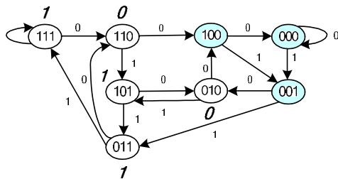
Fig. 5 The combination constraints
