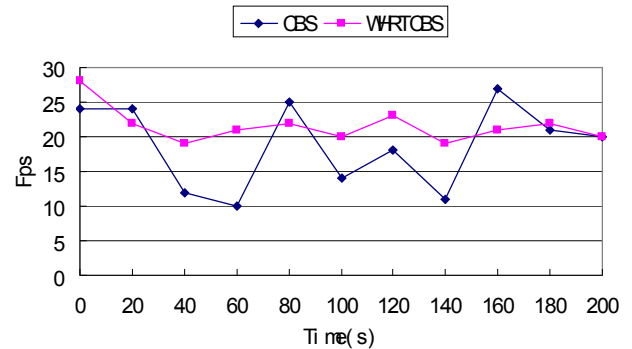
Fig. 8 Middle overloads
