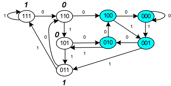
Fig. 3 The state transition diagram of (2, 3)
