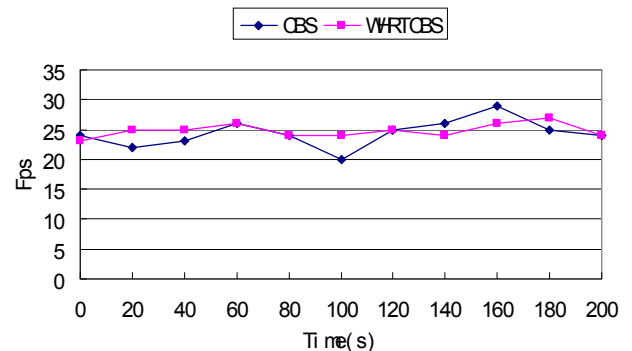
Fig. 9 Light overloads
