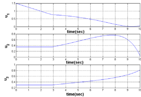
Fig. 4 Control inputs
