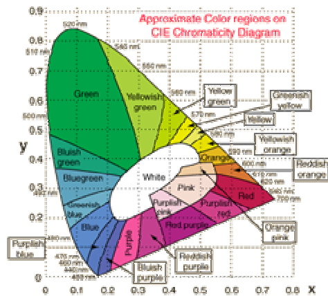
Fig. 2 Approximate colors on CIE chromaticity diagram [10]
