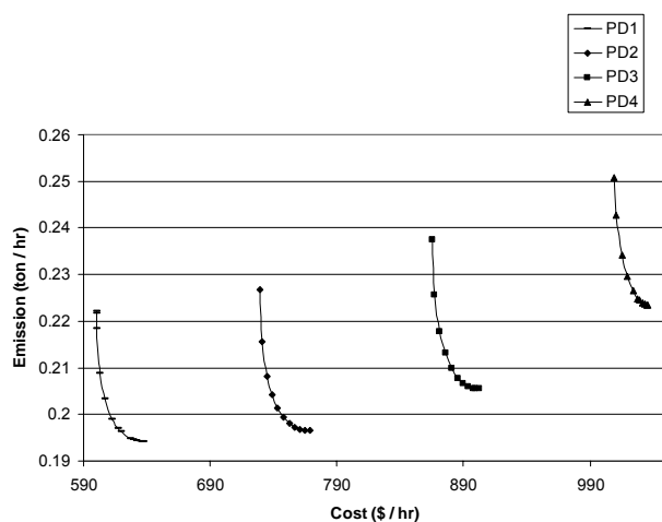
Fig. 2 Pareto Fronts for Different Loading Conditions
