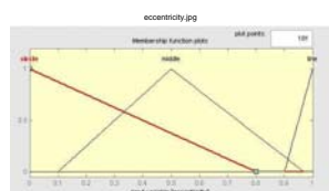
Fig. 4. Example of Triangular Membership Function for Eccentricity
