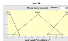
Fig. 7. Example of Mixed Triangular-Trapezoids Membership Function
