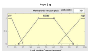
Fig. 6. Example of Trapezoids Membership Function
