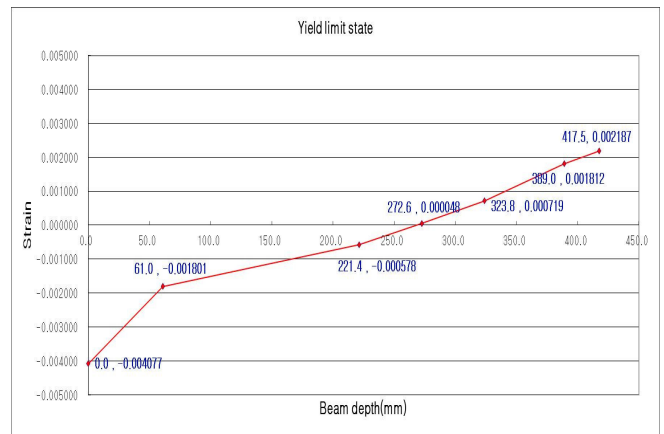
Fig. 8 Transition of Strain in Yield Limit State of Specimen No. 1
