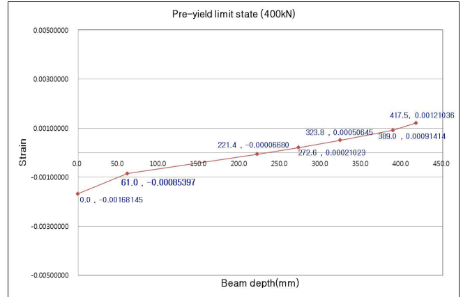
Fig. 7 Transition of Strain in Pre-Yield Limit State of Specimen No. 1(400kN)
