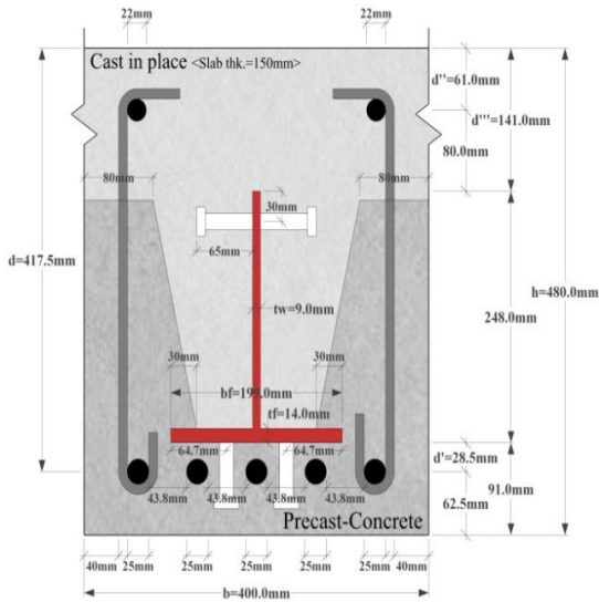
Fig. 1 Detailed Cross-Section of a Specimen
