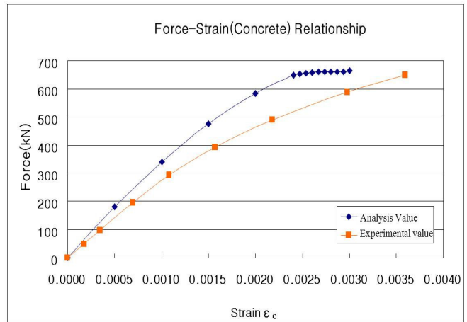
Fig. 4 Force-Strain Relationship for Specimen No. 1
