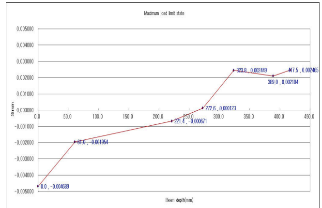
Fig. 13 Transition of Strain in Maximum Load Limit State of Specimen No. 2
