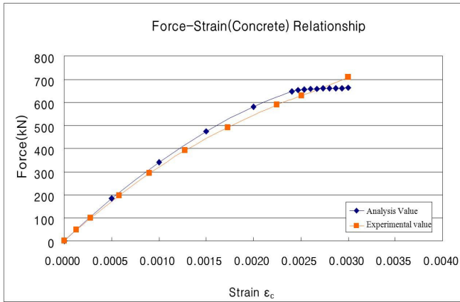
Fig. 5 Force-Strain Relationship for Specimen No. 2
