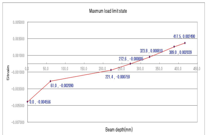
Fig. 9 Transition of Strain in Maximum Load Limit State of Specimen No. 1
