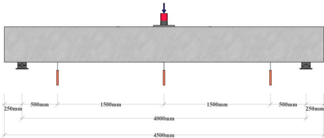
Fig. 2 Loading Method
