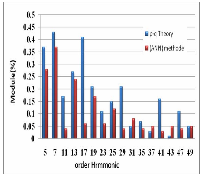
Fig.7. Harmonic spectrum of supply current Phase 'a'
