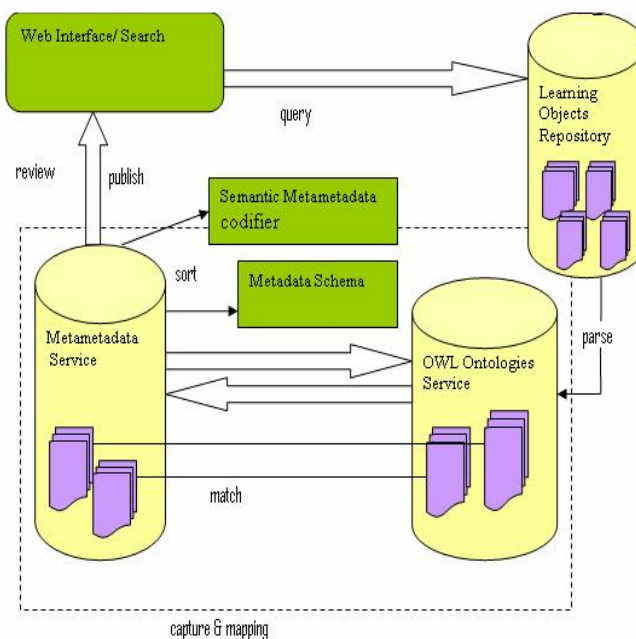
Fig. 4 OMESCOD Architecture
