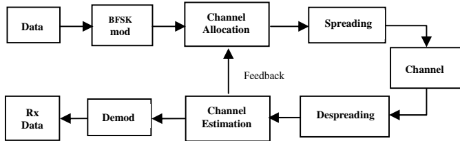
Fig. 4. Block diagram of system model for DFH.
