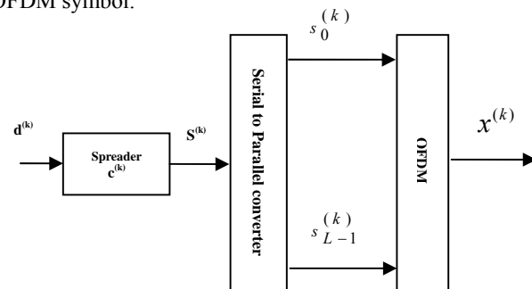
Fig. 3. Multi-carrier spread spectrum signal generation
