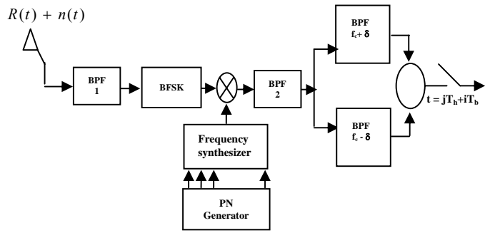
Fig. 1. Block diagram of the SFH/BFSK receiver system.
