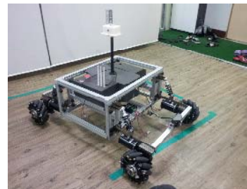
Fig. 1 Omnidirectional Robot used in experiment
