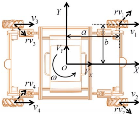
Fig. 3 Omnidirectional mecanum wheel robot Kinematics
