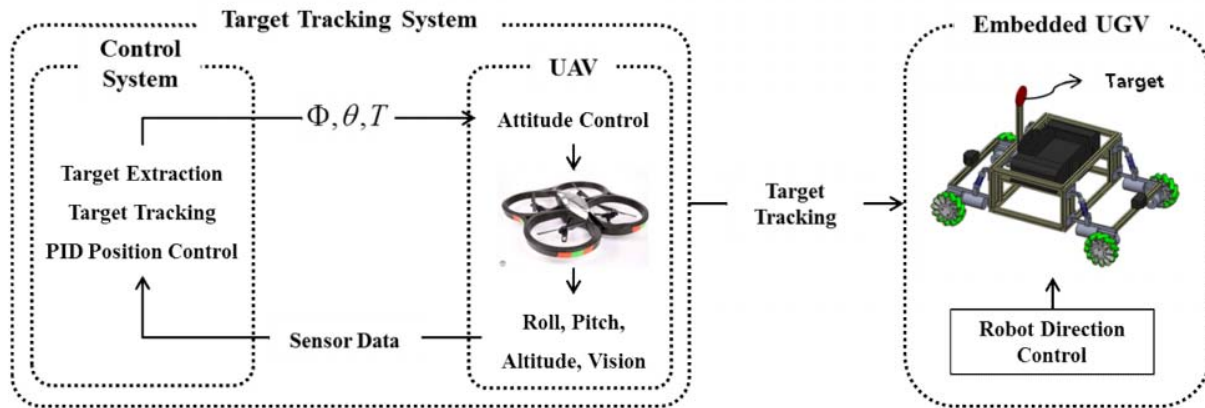
Fig. 2 Overall system configuration
