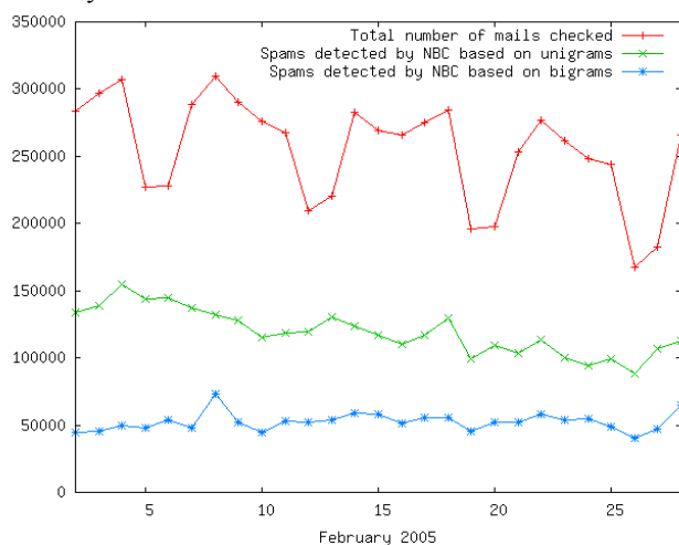
Fig.2 Performance of naïve Bayesian classifiers working at CERN
