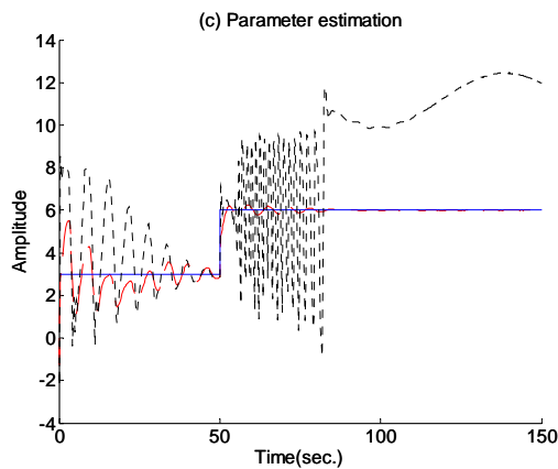
Fig. 2 Parameter estimate using the proposed adaptive observer (dashed) vs. the method in [6] (dotted)
