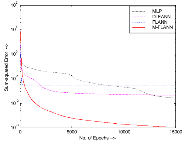
Fig. 6 Comparison of Convergence Speed of ANN Models for a Simulated Continually Stirred Tank Heater
