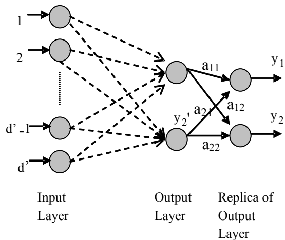
Fig. 4 M-FLANN, Equivalent Feedforward Neural Net
