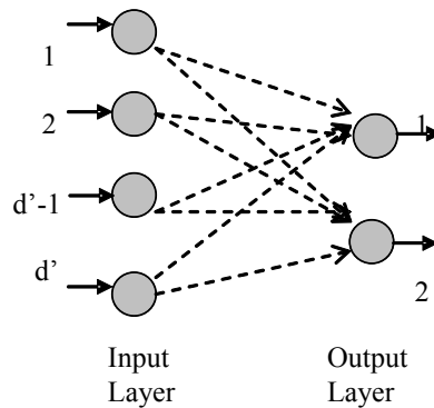
Fig. 2 Functional Link Artificial Neural Network (FLANN)
