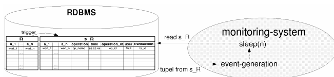
Fig. 3 Monitoring: Triggers and Polling
