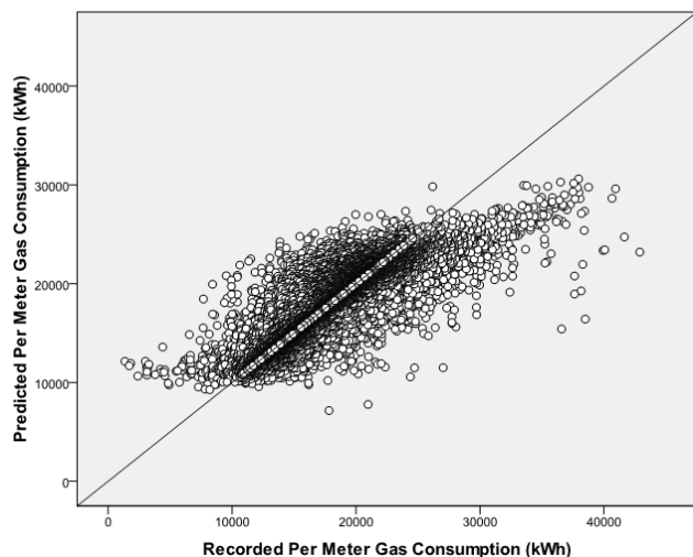
Fig. 4 Plot of predicted values against actual values
