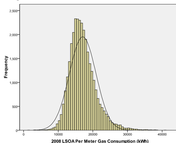
Fig. 1 Distribution of LSOA per meter gas consumption (2008)
