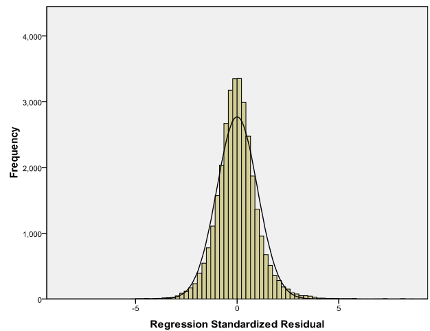
Fig. 2 Histogram of residuals from regression model
