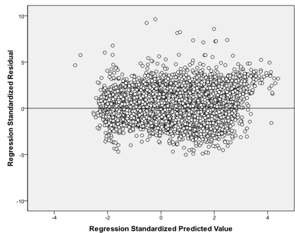
Fig. 3 Plot of model residuals against predicted values
