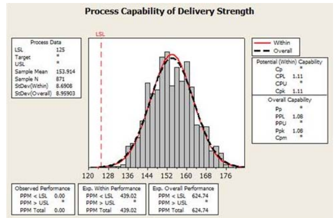
Fig. 14 Process capability based on strength quality (after improvement)
