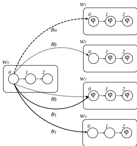
Fig. 1. Example of a telephone game
