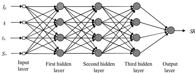
Fig. 4 Multilayer perceptron neural network model structure
