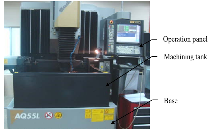
Fig. 1 Experimental setup of electrical discharge machining.
