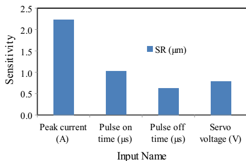
Fig. 7 Sensitivity analysis for surface roughness
