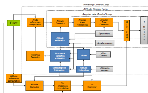
Fig. 3 Data transfer within the AR Drone [11]
