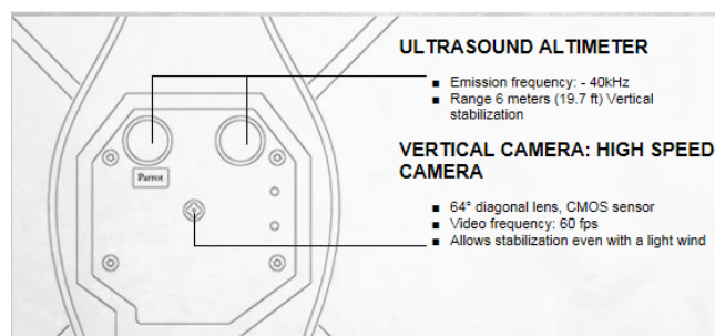
Fig. 2 Parrot AR. Drone bottom sensors [1]
