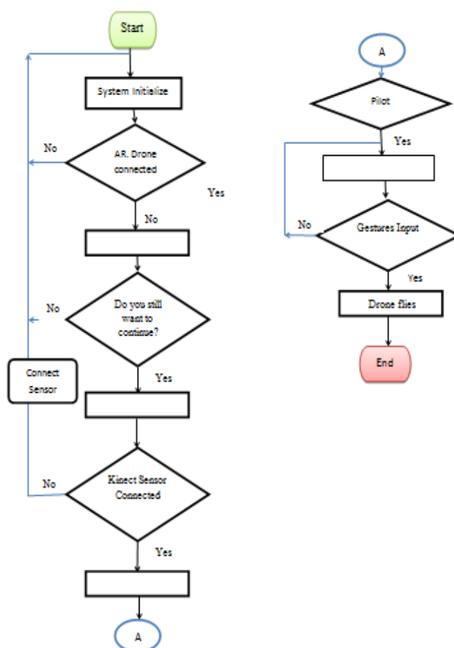
Fig. 6 The System State Diagram
