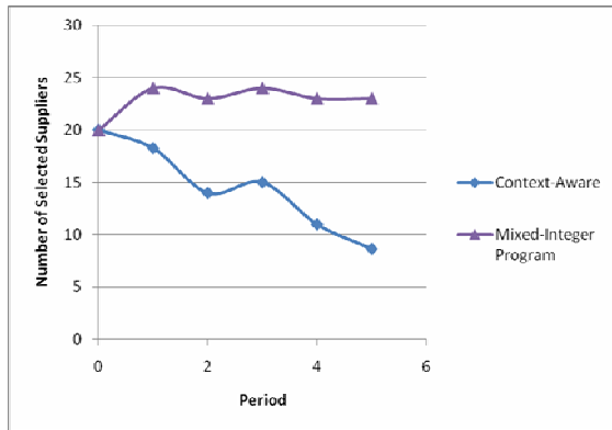
Fig. 4: Number of selected suppliers per period
