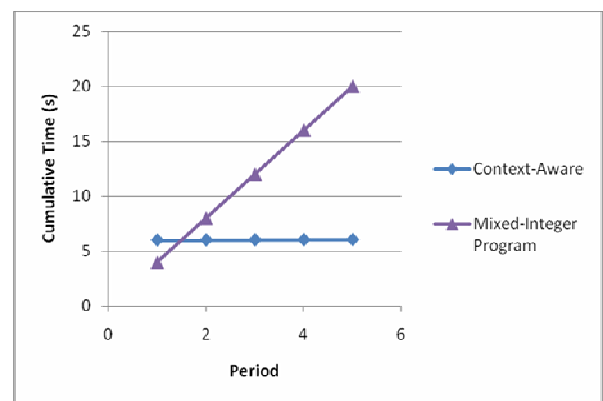
Fig. 8: Cumulative computational time per period
