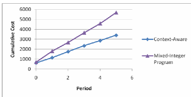
Fig. 6: Cumulative cost per period
