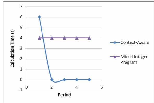
Fig. 7: Computational time per period
