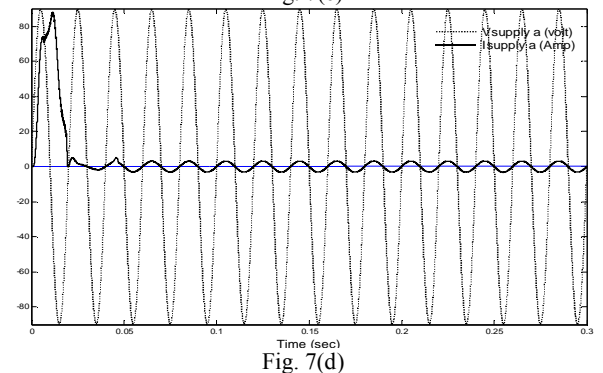
Fig. 7 The simulation results for (a) phase load current, (b) phase filter current, (c) neutral current, and (d) supply voltage and current
