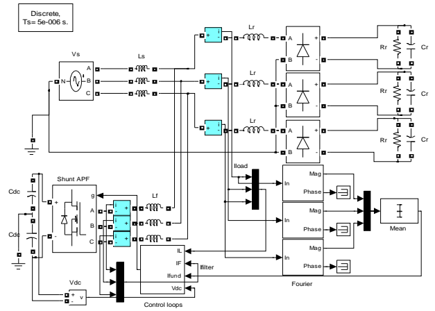
Fig. 5 The test system simulation with balanced nonlinear loads
