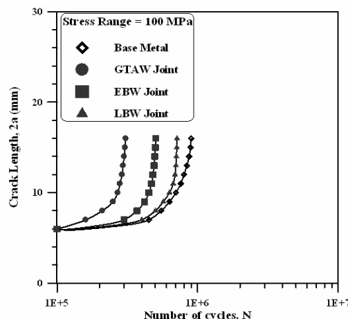
Crack growth curves at 100 MPa
