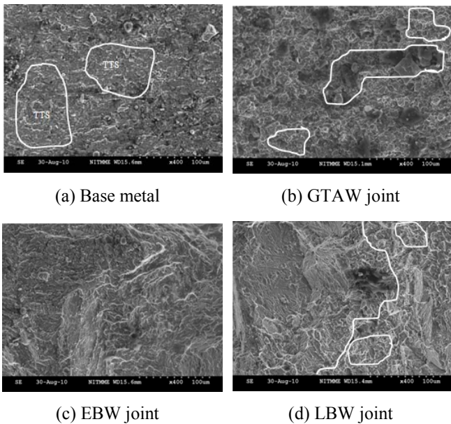
Fig.9 Fractographs of FCI region
