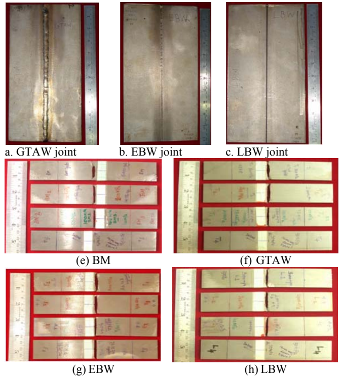
Fig. 4 Photographs of welded joints and CCT specimen (a-c: joints; d-g: CCT specimens)
