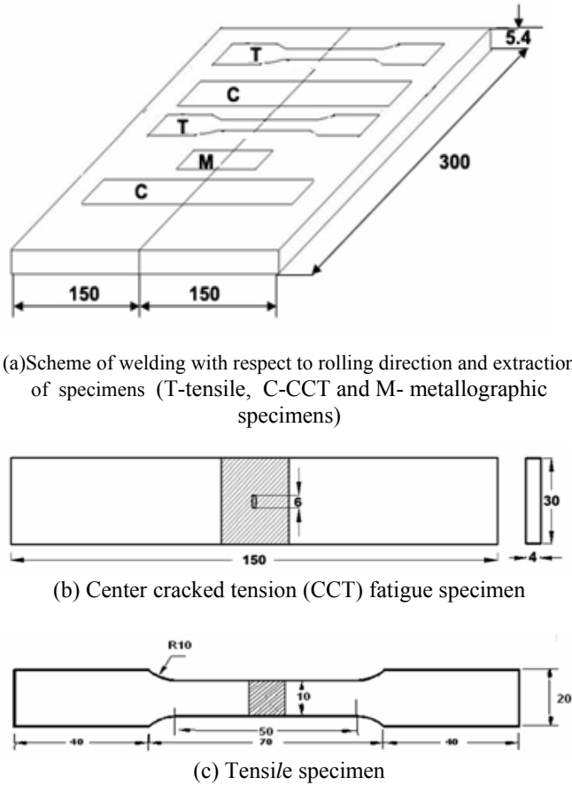
All dimensions are in 'mm' Fig.3 Joint and specimen dimensions
