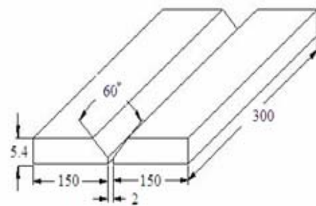
(a) Single 'V' butt joint (for GTAW)
