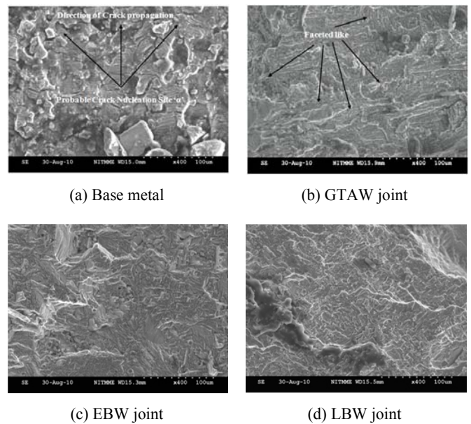
Fig.10 Fractographs of FCP region
