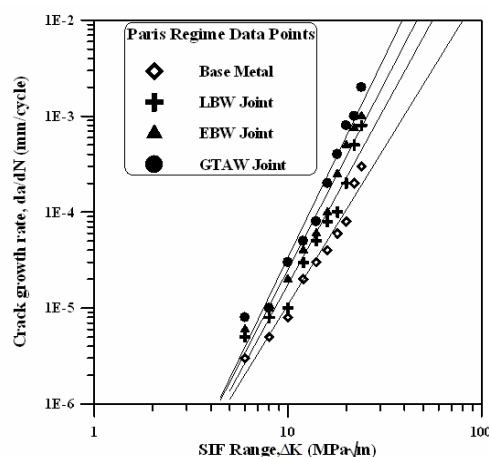
Fig.6 Effect of welding processes on fatigue crack growth rate
