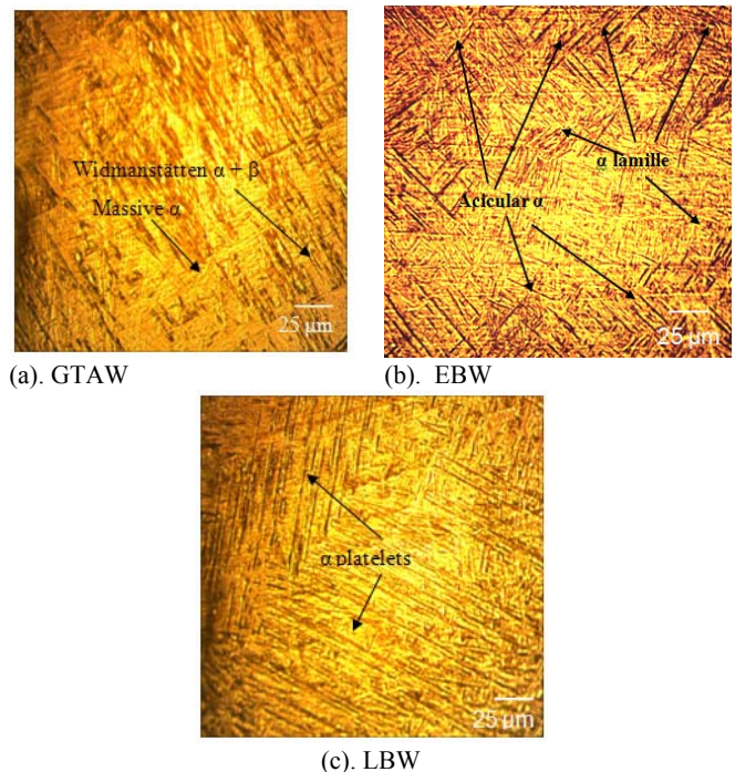
Fig.8 Optical micrograph of weld metals
