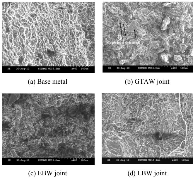
Fig.11 Fractographs of FF region
