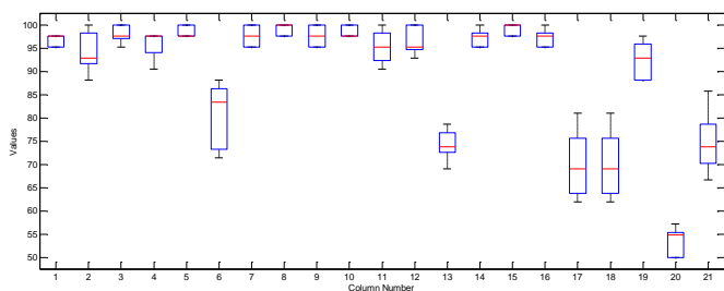
Fig. 3 CLASSIFICATION ACCURACY OF THE 2-STYLES CLASSIFIER
