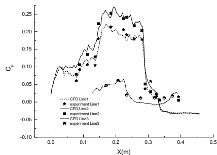
Fig. 11 Ma = 5.993\alpha = 4\beta = 0
