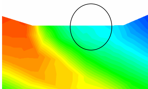
Fig.12 Pressure distribution at Ma = 5.993\alpha = 4\beta = 4
