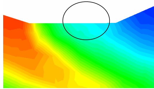
Fig. 8 Pressure distribution at Ma=6
