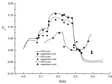
Fig.5 Ma = 4.937\alpha = 0\beta = 0
