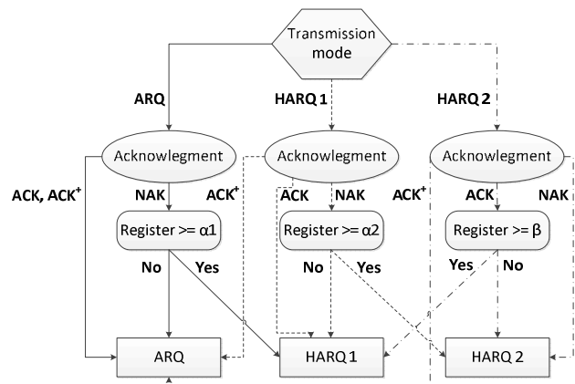
Fig. 2 Logic of transmitter in our proposal
