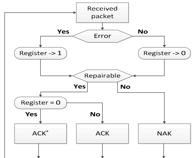
Fig. 1 Logic of receiver in our proposal
