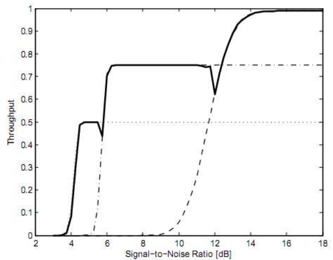
Fig. 4 Dependence of relative throughput on SNR
