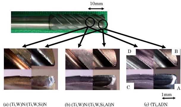
Fig. 2 Tool wear at a cutting speed of 3.33 m/s and a cutting length of 36.4 m
