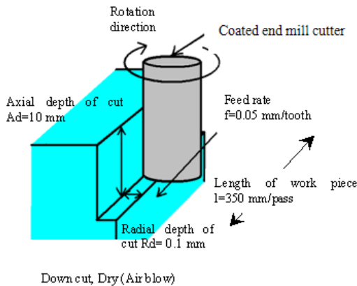
Fig. 1 Schematic view of the milling test
