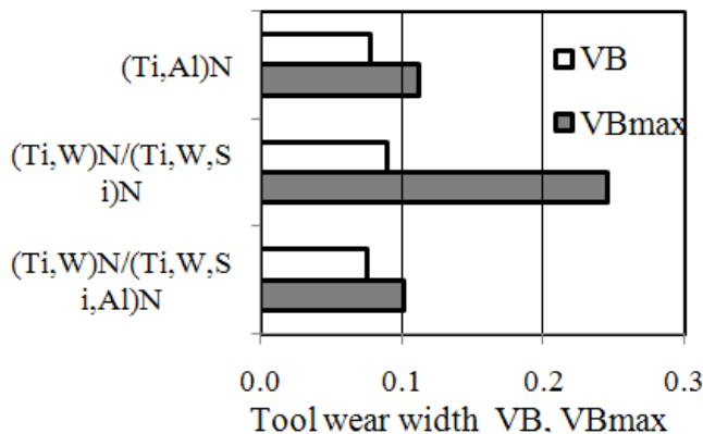
Fig. 4 Tool wear width at a cutting speed of 3.33 m/s and a cutting length of 36.4 m
