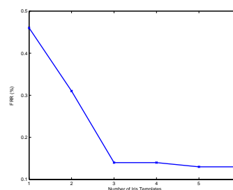
Fig. 12 FRR vs Number of training sample
