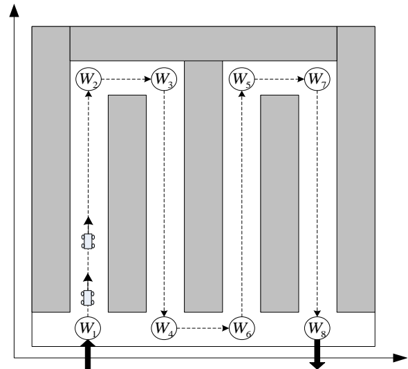
Fig. 3. Greenhouse ground plan.
