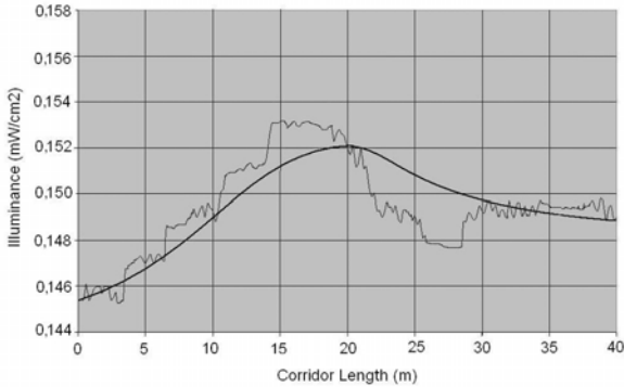
Fig. 10. Illuminance for wavelength of 660nm with closed windows.
