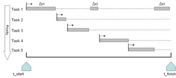
Fig. 2. Jobs are executed in a multi tasks Operating System
