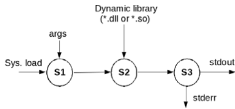
Fig. 4. State transitions in a dynamic linking system
