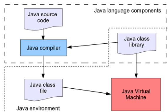
Fig. 1. Components in Java technology architecture
