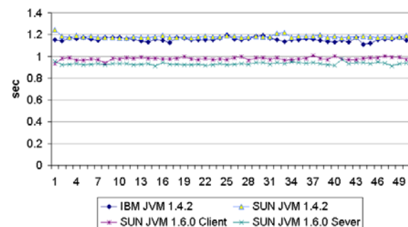
Fig. 11. Runtime comparison, Hanoi 27 towers. The lower the better.
