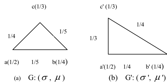
Fig. 1 Weak Isomorphism
