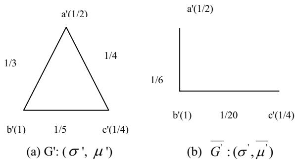
Fig. 8 Fuzzy Graph G' and its complement \overline{G}'
