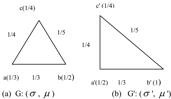
Fig. 2 Co-weak Isomorphism
