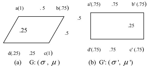
Fig. 4 Graphs of same order but not weak isomorphic The above two fuzzy graphs are of order 3 but they are not weak isomorphic.
