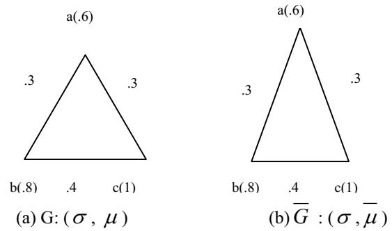
Fig. 11 Self complementary fuzzy graph
