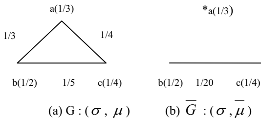
Fig. 7 Fuzzy Graph G and its complement \overline{G}
