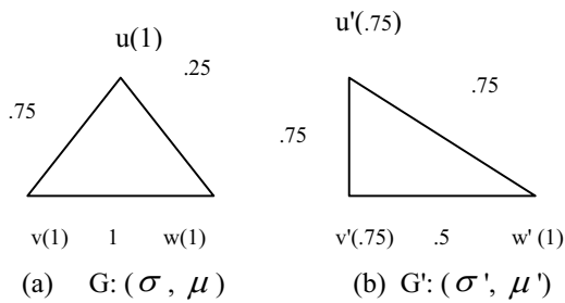
Fig. 5 Graphs of same size but not co- weak isomorphic Definition 3.15[3]: Let G: (\sigma, \mu) be a fuzzy graph. The
