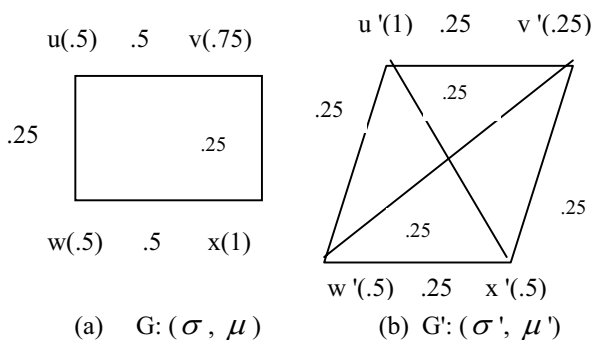
Fig. 6 Graphs preserving the degree of the vertices
