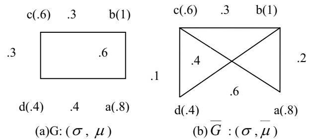
Fig. 12 Fuzzy graph not self complementary.
