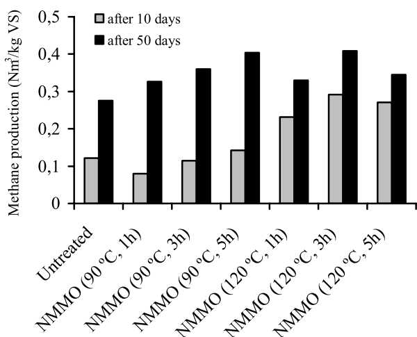
Fig. 2 Accumulated methane production (Nm 3 /kg VS) after 10 (gray bars) and 50 days (black bars) of digestion from untreated OPEFB and treated OPEFB using 85% NMMO
