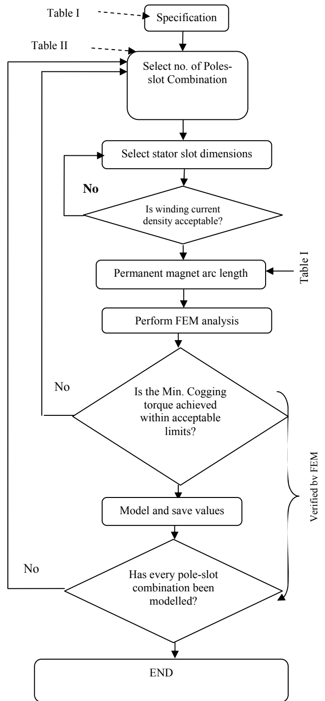
Fig. 2 Logic flowchart applied to each part of the DSCR machine to select the minimum cogging torque
