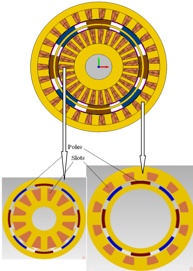
Fig. 1 Integrated machine design
