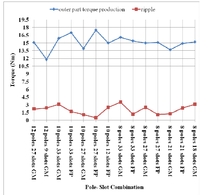
Fig. 9 The electromagnetic torque and the peak to peak ripple torque of the DSCR machine (outer part)
