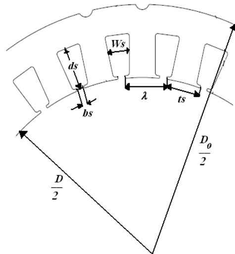
Fig. 4 The stator configuration
