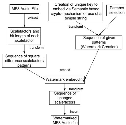
Fig. 1 Main algorithm
