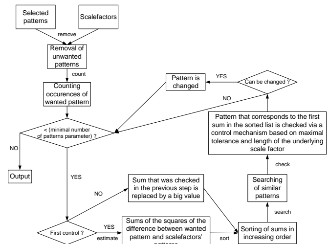
Fig. 2 Watermark embedding
