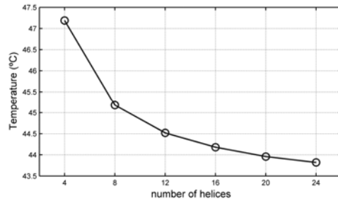
Fig. 13 Maximum temperature after 15 minutes at 25 V.
