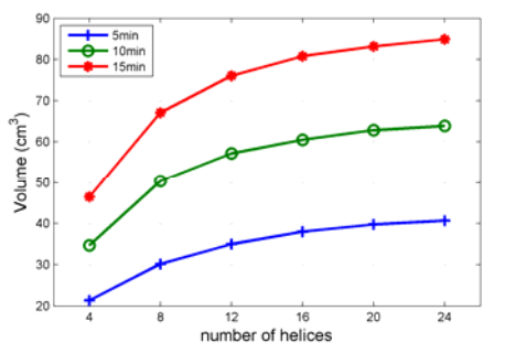
Fig. 16 Lesion volume obtained for each stent model after 5, 10 and 15 minutes at 75 V
