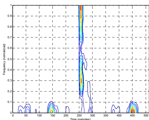
Figure 3. Time-frequency distribution for the RDPW signal.
