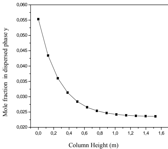
Fig 3 Variation of the along the column ( V_c=2.10\text{mm/s} , V_d=4.75\text{mm/s} E_z = 1.66 \cdot 10^{-3} \text{m}^2/\text{s} or \text{Ped}=0.023 )
