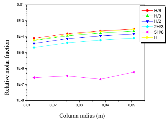
Fig 8 Profile of the relative fraction with zero gradient at the wall (48 elements)
