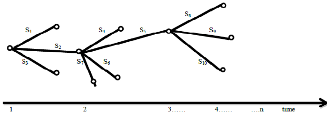
Fig. 1 Decision Tree probabilities and new strategies
