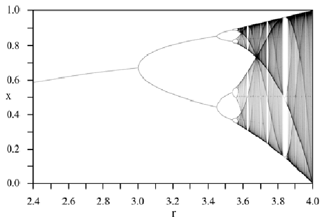
Fig. 2 The famous logistic map bifurcation diagram
