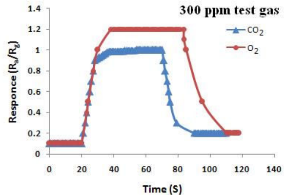
Fig. 7 Response transients of the ZnO nanowires array films to 300ppm various gases at 100 °C
