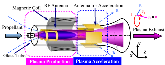
Fig. 1 Concept of Lissajous acceleration-type plasma thruster
