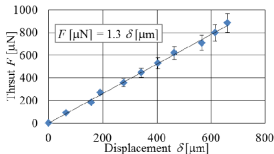
Fig. 6 Result of thrust stand calibration
