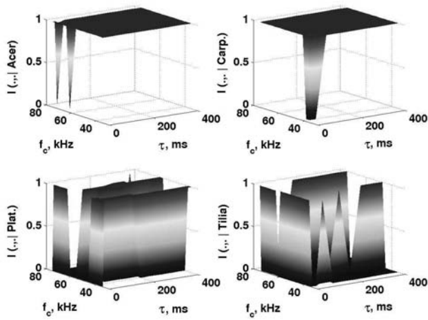
Fig. 4. Class separation performance with LPF structure (2).
