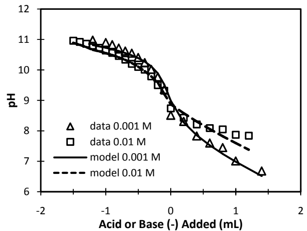
Fig. 8 Potentiometric titration data of clayey sediments at two ionic strengths with TL-SCM simulations
