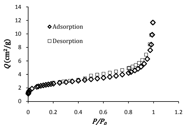
Fig. 3 N 2 -isotherm for activated sediment sample (fraction 30/50)
