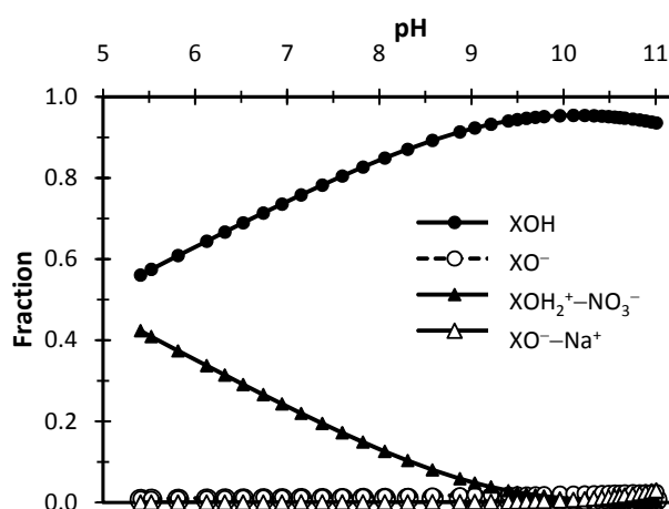
Fig.10 Surface speciation of clayey sediments in 0.01 M NaNO_3 from triple layer model calculations using equilibria and constants given in Equations (3)-(6)
