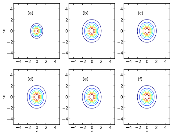
Fig. 1. results for each iterations : (a) i = 0 , (b) i = 10 , (c) i = 20 , (d) i = 30 , (e) i = 35 , (f) i = 56 .
