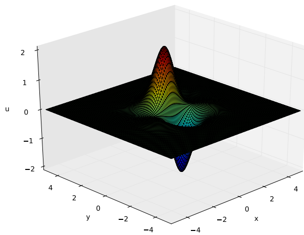
Fig. 3. the initial profile of 5 \operatorname{sech}^2(\sqrt{x^2 + y^2}) \cos(x) \sin(y)
