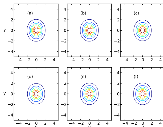
Fig. 6. time evolution of the solitary wave solution: (a) t = 0 , (b) t = 2 , (c) t = 4 , (d) t = 6 , (e) t = 8 , (f) t = 10
