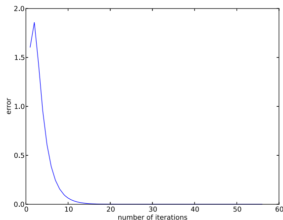
Fig. 2. shows error for each iteration
