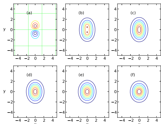
Fig. 4. results for each iterations : (a) i = 0 , (b) i = 1 , (c) i = 2 , (d) i = 3 , (e) i = 4 , (f) i = 58 .
