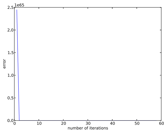
Fig. 5. shows error for each iteration
