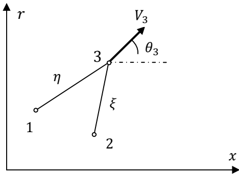
Fig. 3 Intersection of two characteristics
