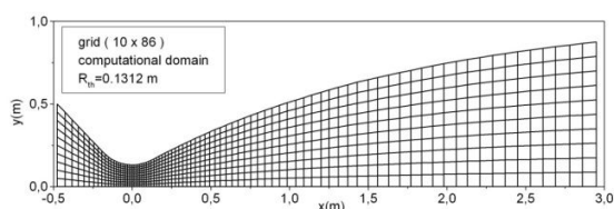
Fig. 16 Grid in the nozzle
