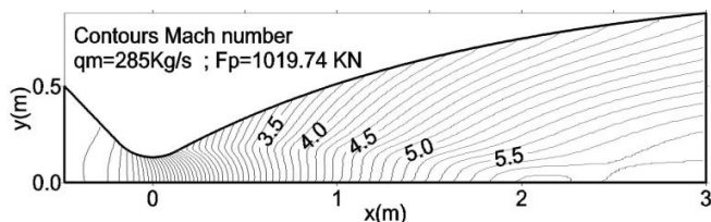
Fig. 17 Mach contours in the nozzle
