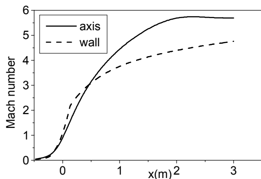
Fig. 18 Mach number evolution in the nozzle
