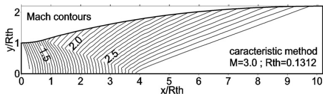
Fig. 12 Mach-contours in the diverging of the nozzle
