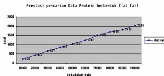
Fig. 9 Execution time for searching protein data flat file database
