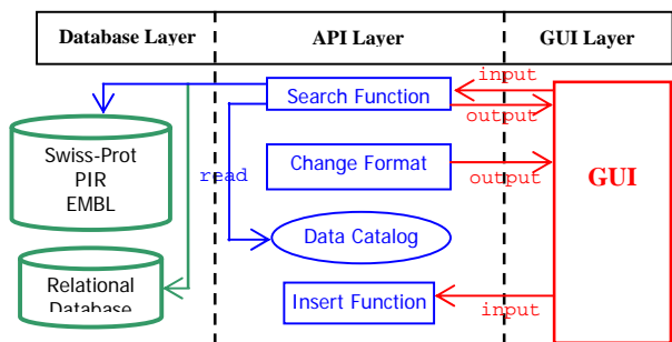
Fig. 4 System's architecture
