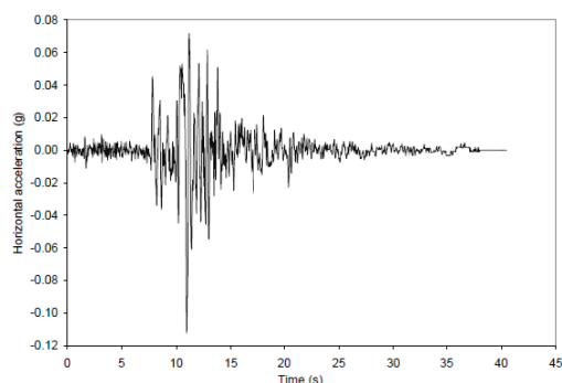
Fig. 1 Horizontal acceleration of the Bam 2003 earthquake
